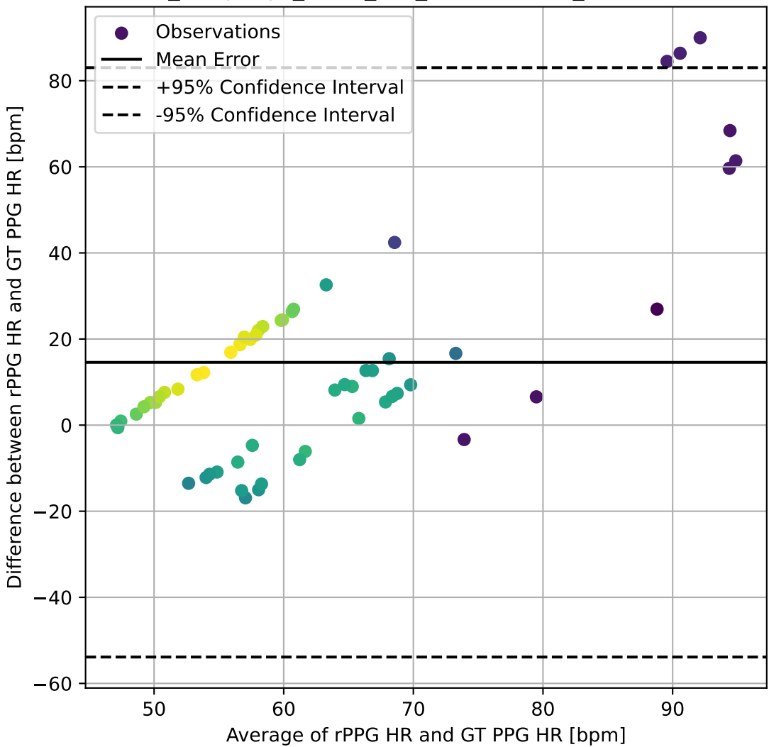
PURE_DeepPhys_PURE_FFT_BlandAltman_DifferencePlot
