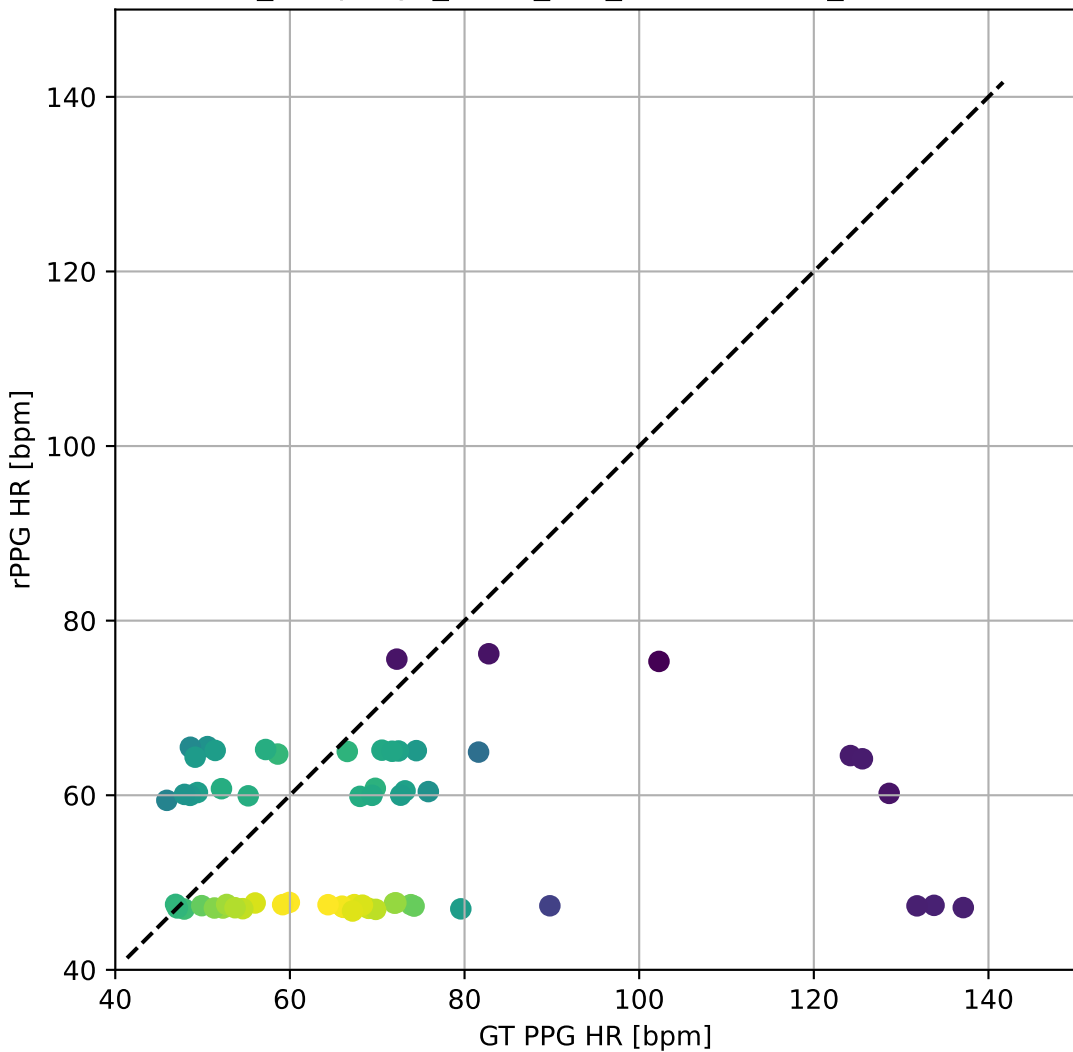
PURE_DeepPhys_PURE_FFT_BlandAltman_ScatterPlot
