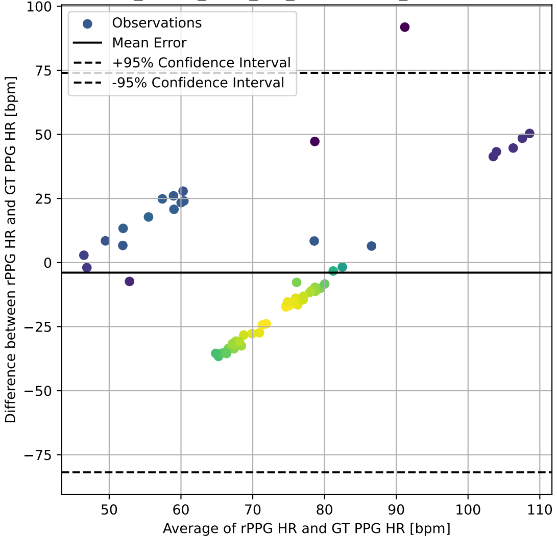
PURE_TSCAN_PURE_FFT_BlandAltman_DifferencePlot
