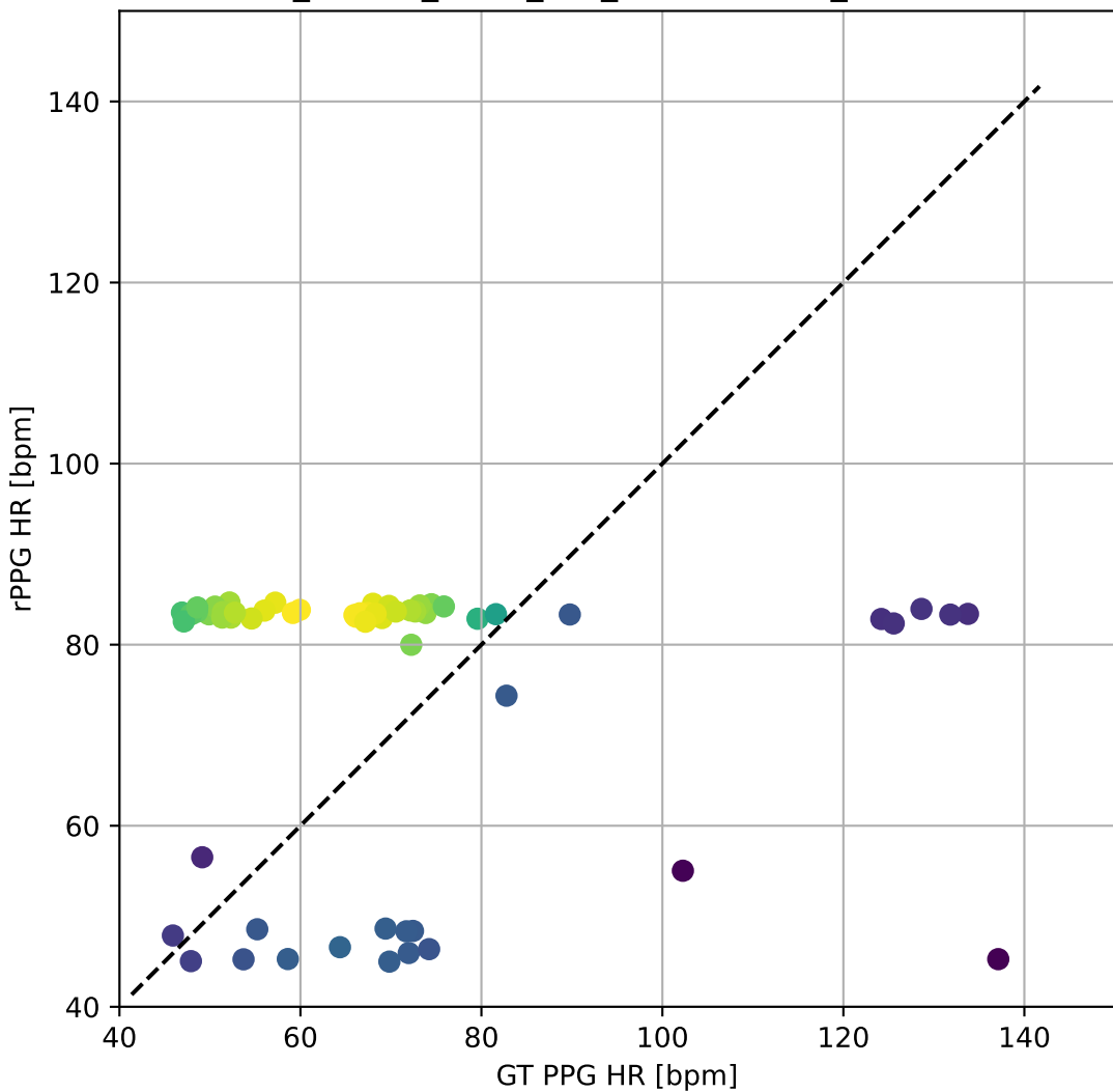
PURE_TSCAN_PURE_FFT_BlandAltman_ScatterPlot
