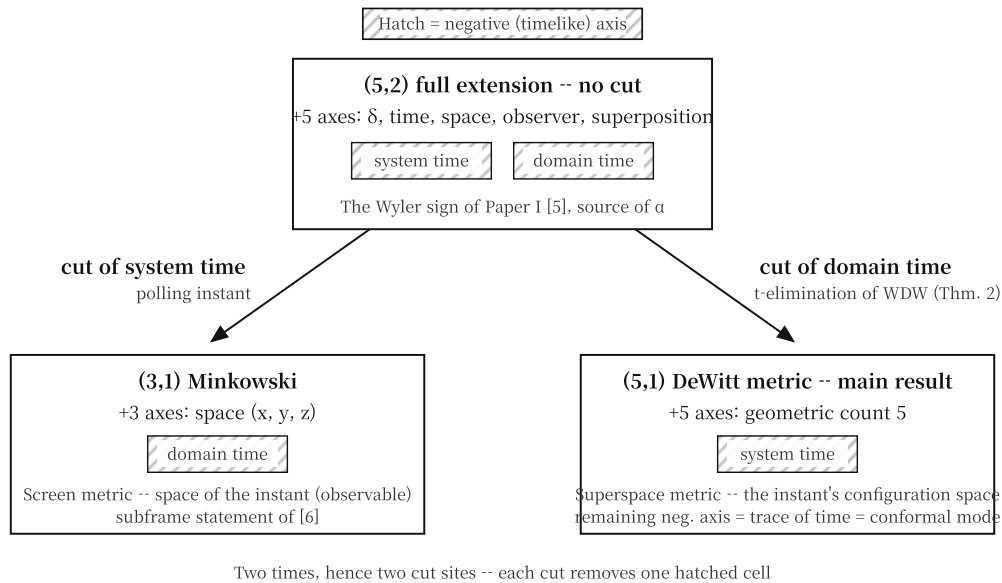
Figure 3. Two cuts, two signatures - the 2 negative axes of the parent (5,2) are the two times. Cutting the system time leaves observable spacetime (3,1); cutting the domain time (Theorem 2) leaves the DeWitt metric (5,1). The two famous Lorentzian signatures are the two complementary cuts of "which time is fixed to now."
