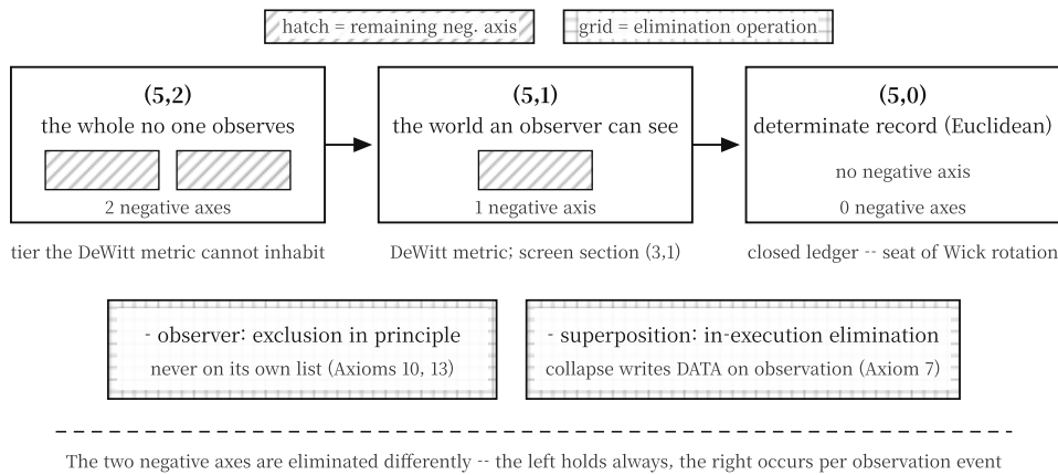
Figure 6. The signature-ladder hypothesis ([6] H-990) - the in-principle exclusion of observer lowers (5, 2) to (5, 1), and the in-execution elimination (collapse) of superposition lowers (5, 1) to (5, 0). Hatched cells are the remaining negative axes.
