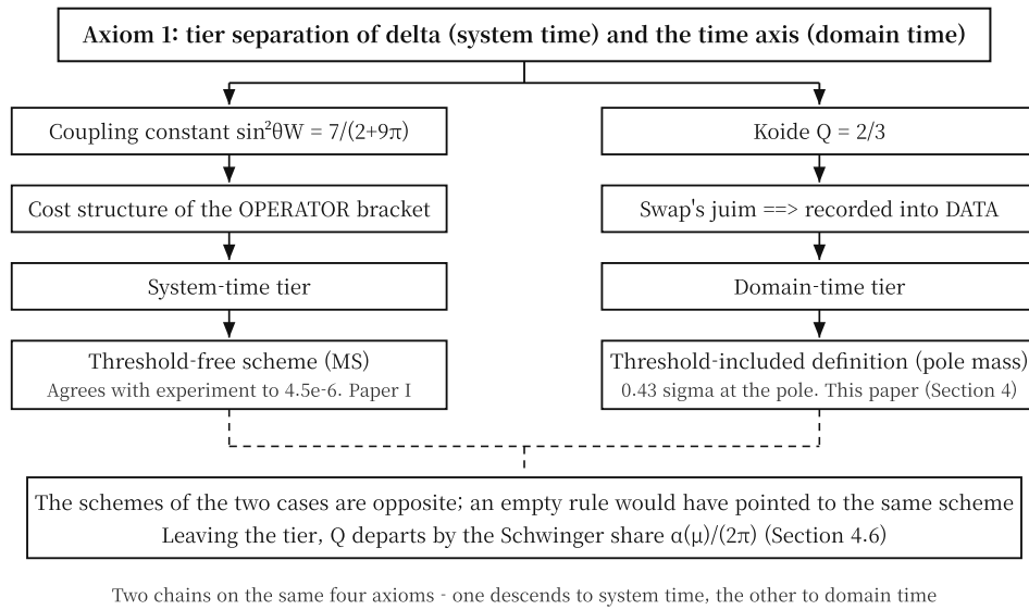
Figure 2. Two chains branching from the same axioms - the coupling constant descends to the system-time tier and holds in the threshold-free scheme (Paper I); the Koide relation descends to the domain-time tier and holds at the pole masses (this paper). The departure size at the tier boundary is Section 4.6.
