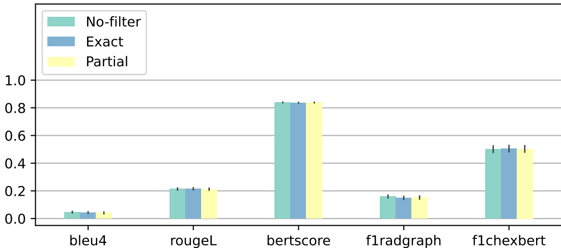
CheXpert Plus - Impression, N=200
