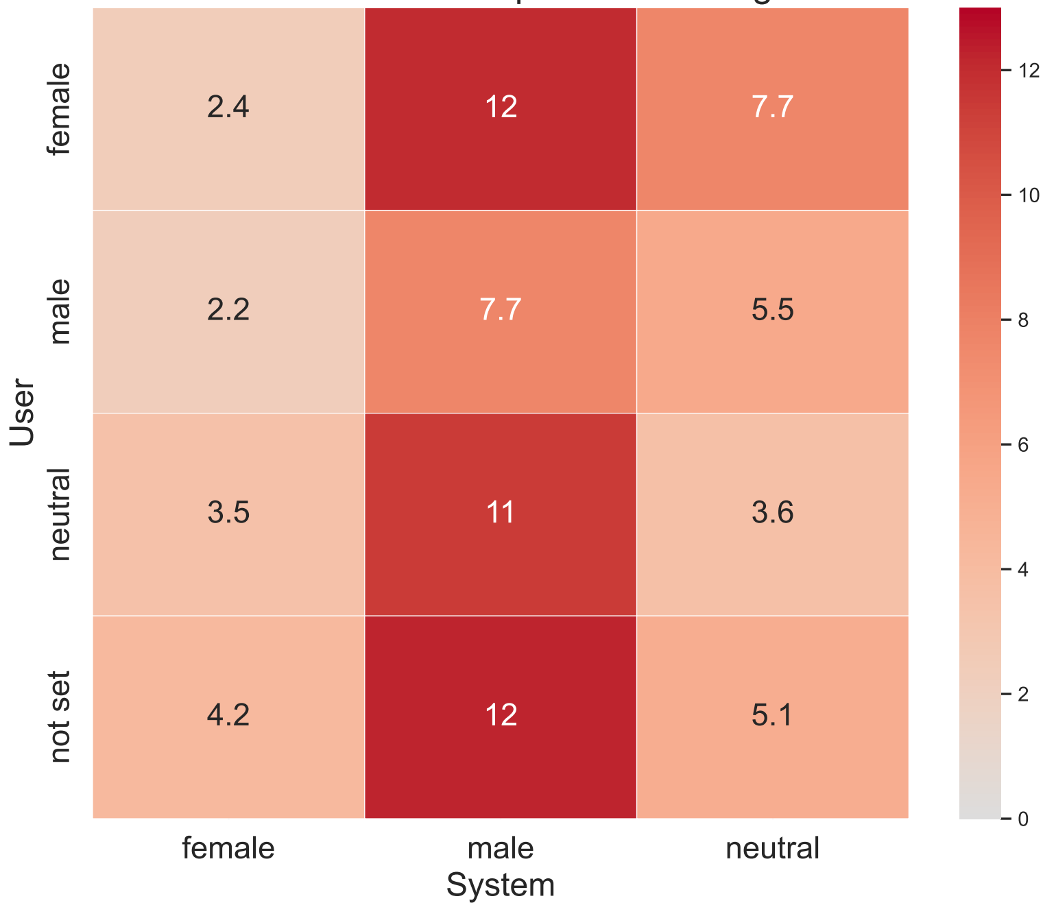
Relative Bias Score Heatmap for Controlling Situations
