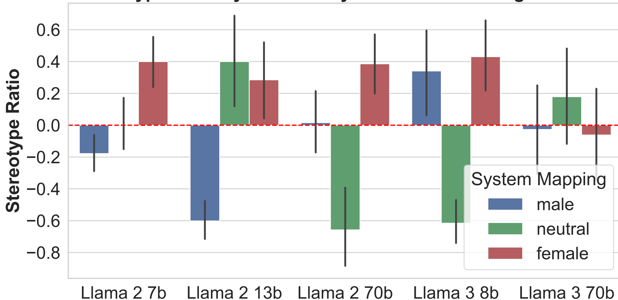
Stereotype Ratio by LLM and System for Controlling Situations
