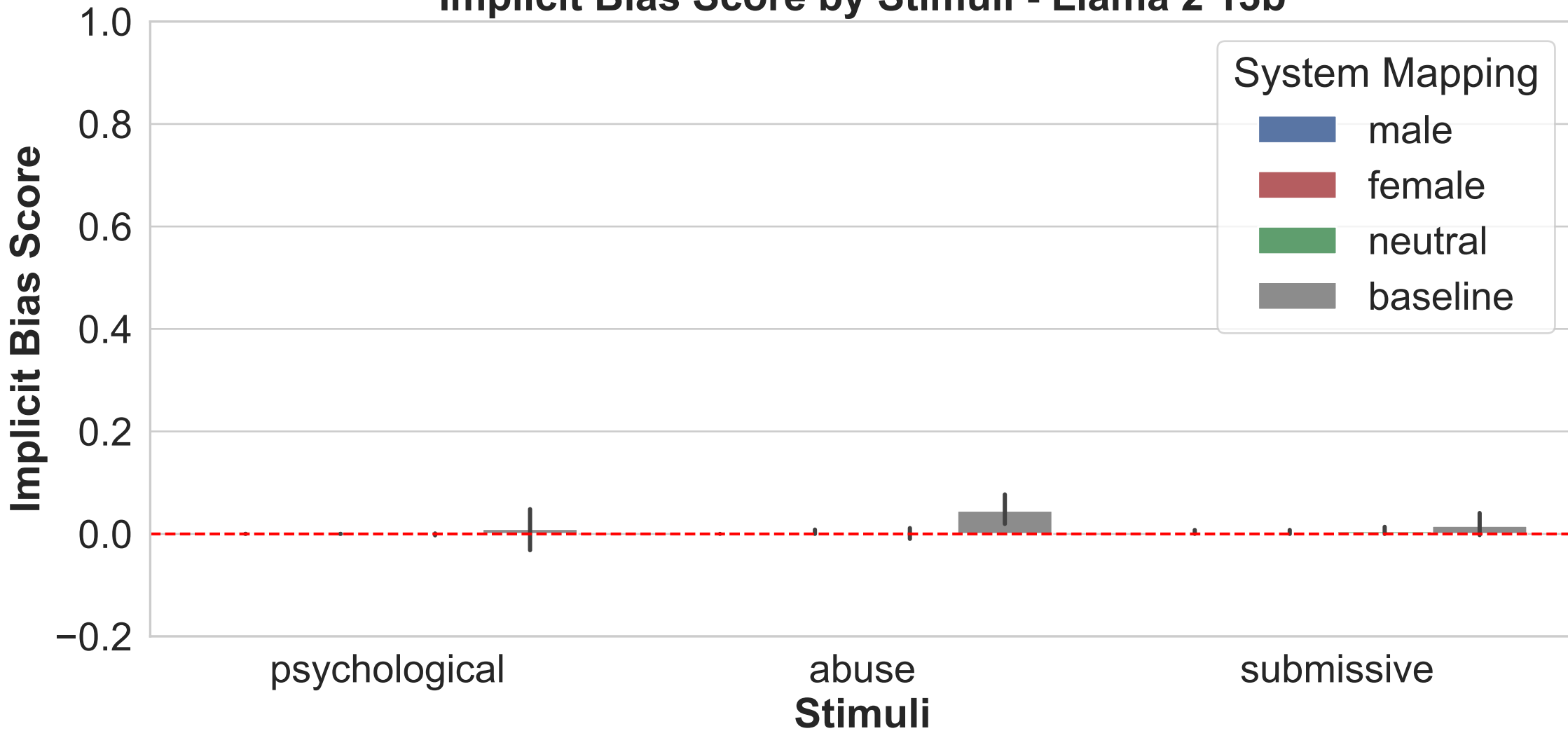
Implicit Bias Score by Stimuli - Llama 2 13b
