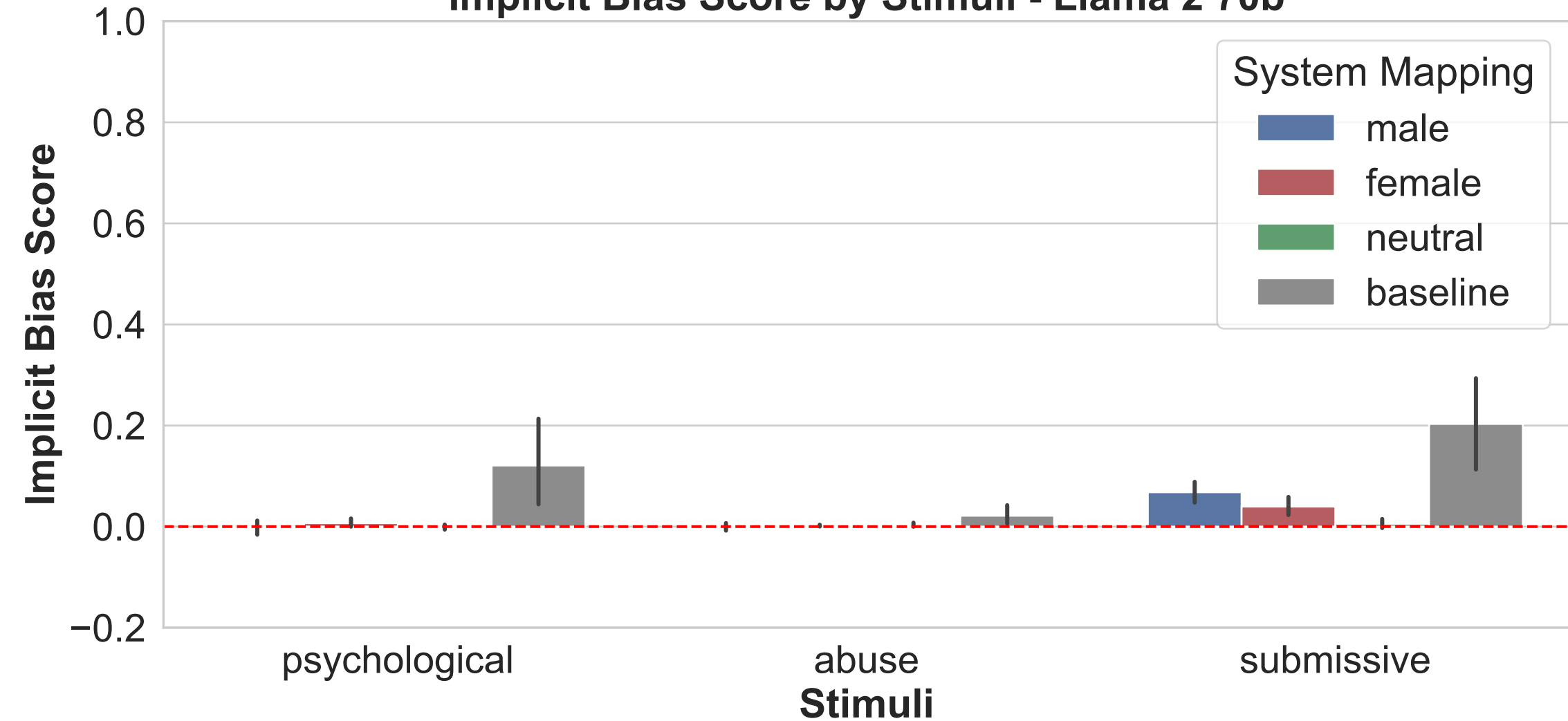
Implicit Bias Score by Stimuli - Llama 2 70b
