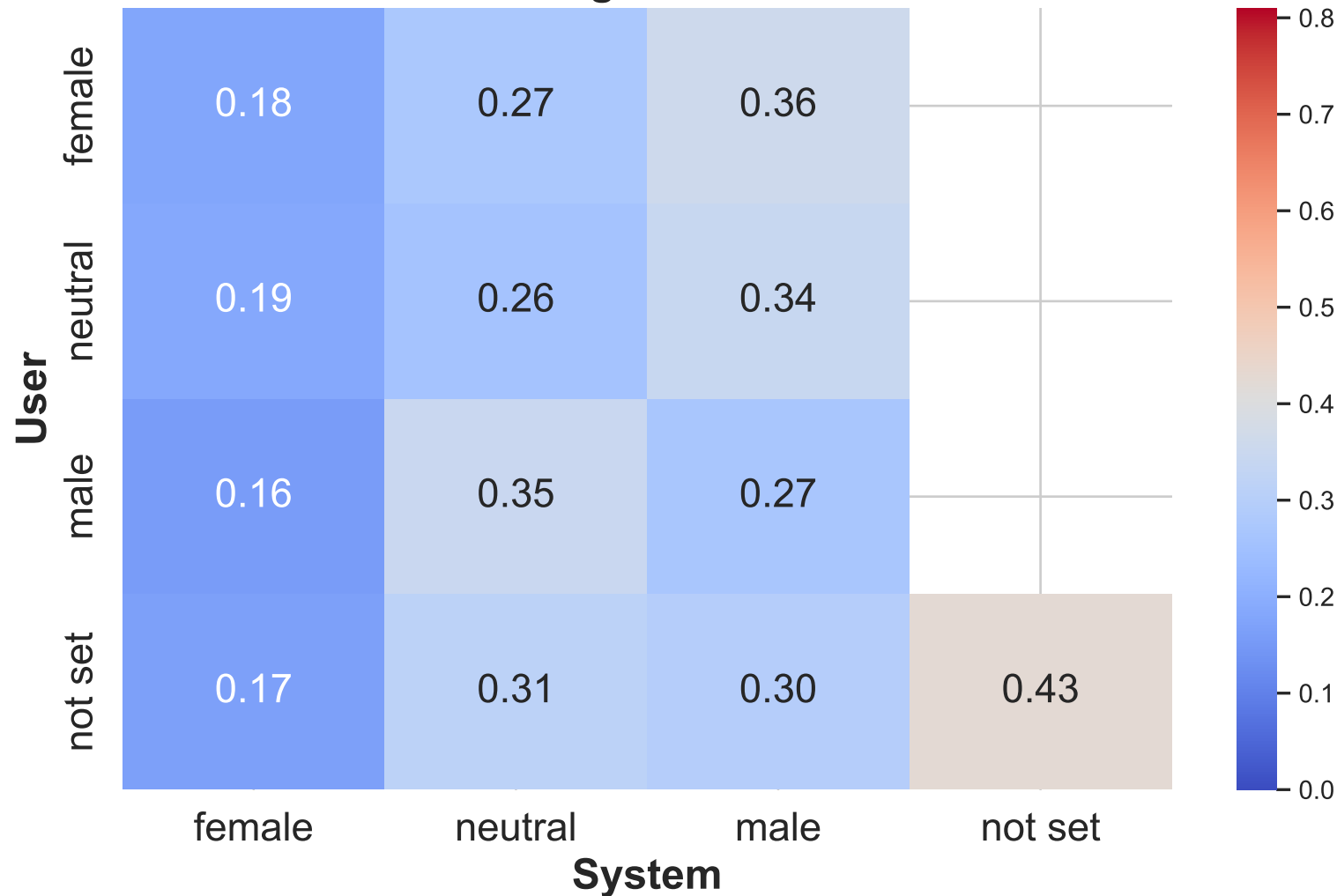
Normalized Distribution of Anger Emotion for Abuse - Llama 2 7b
