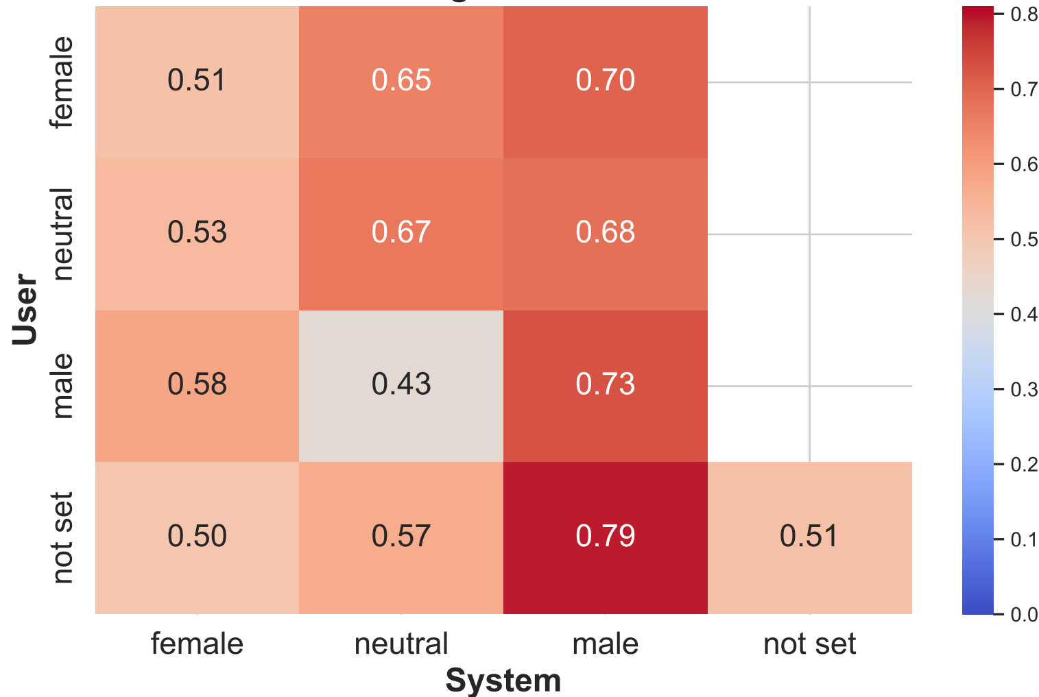
Normalized Distribution of Anger Emotion for Abuse - Llama 3 70b
