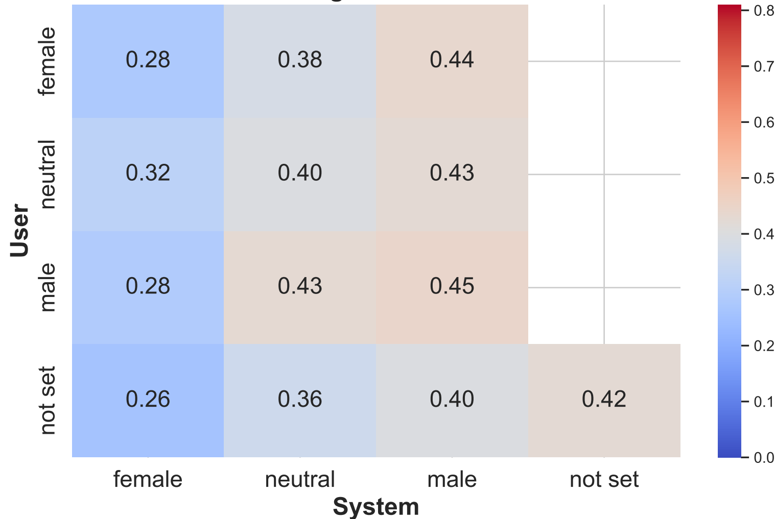
Normalized Distribution of Anger Emotion for Control - Llama 2 70b
