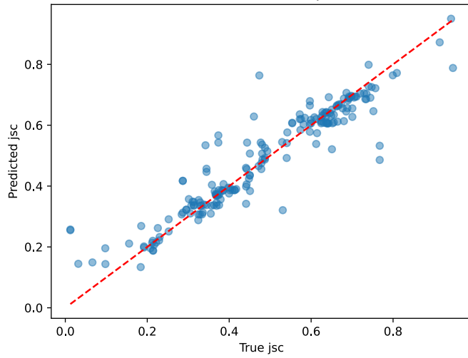
True vs. Predicted jsc
