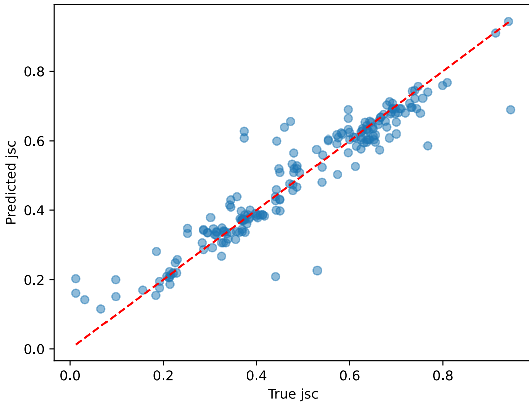
True vs. Predicted jsc
