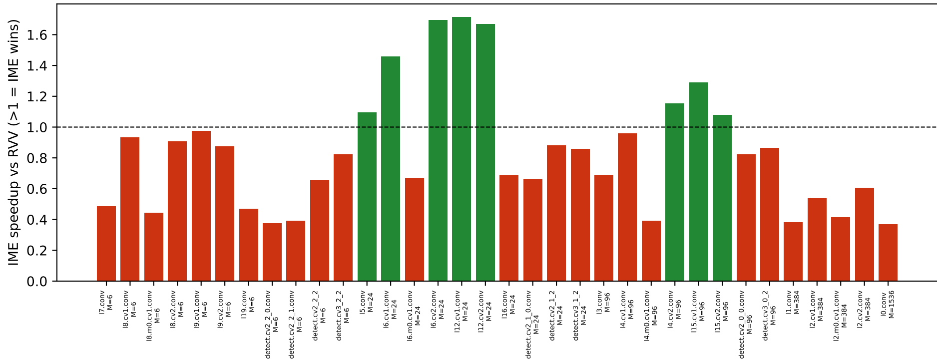
conv2d-on-IME vs RVV per layer (green=IME wins) — bit-exact
