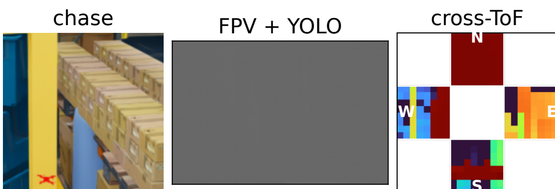
b ROS · loses stability → crash · t=9.0s
