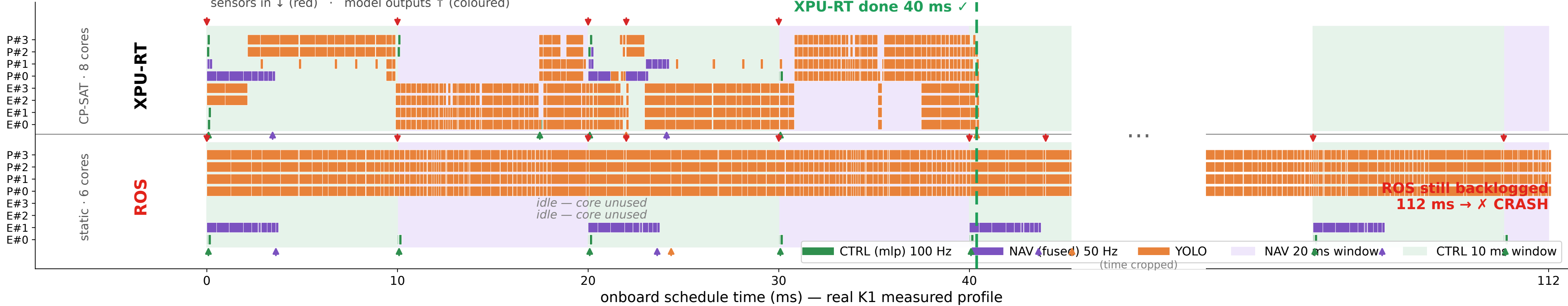
Combined onboard K1 schedule — XPU-RT balances 8 cores and fits the frame; ROS pins 6 cores, serial YOLO overruns → backlog → crash
