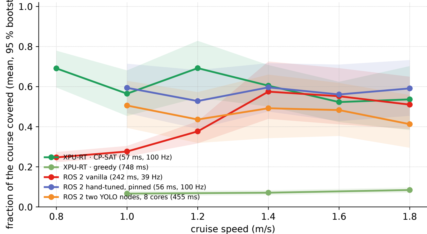
How far each arm gets, graded: course fraction against cruise speed (course A, density 0.30, people 2.4 m, cadence and latency replayed from the K1, one flight per seed)
