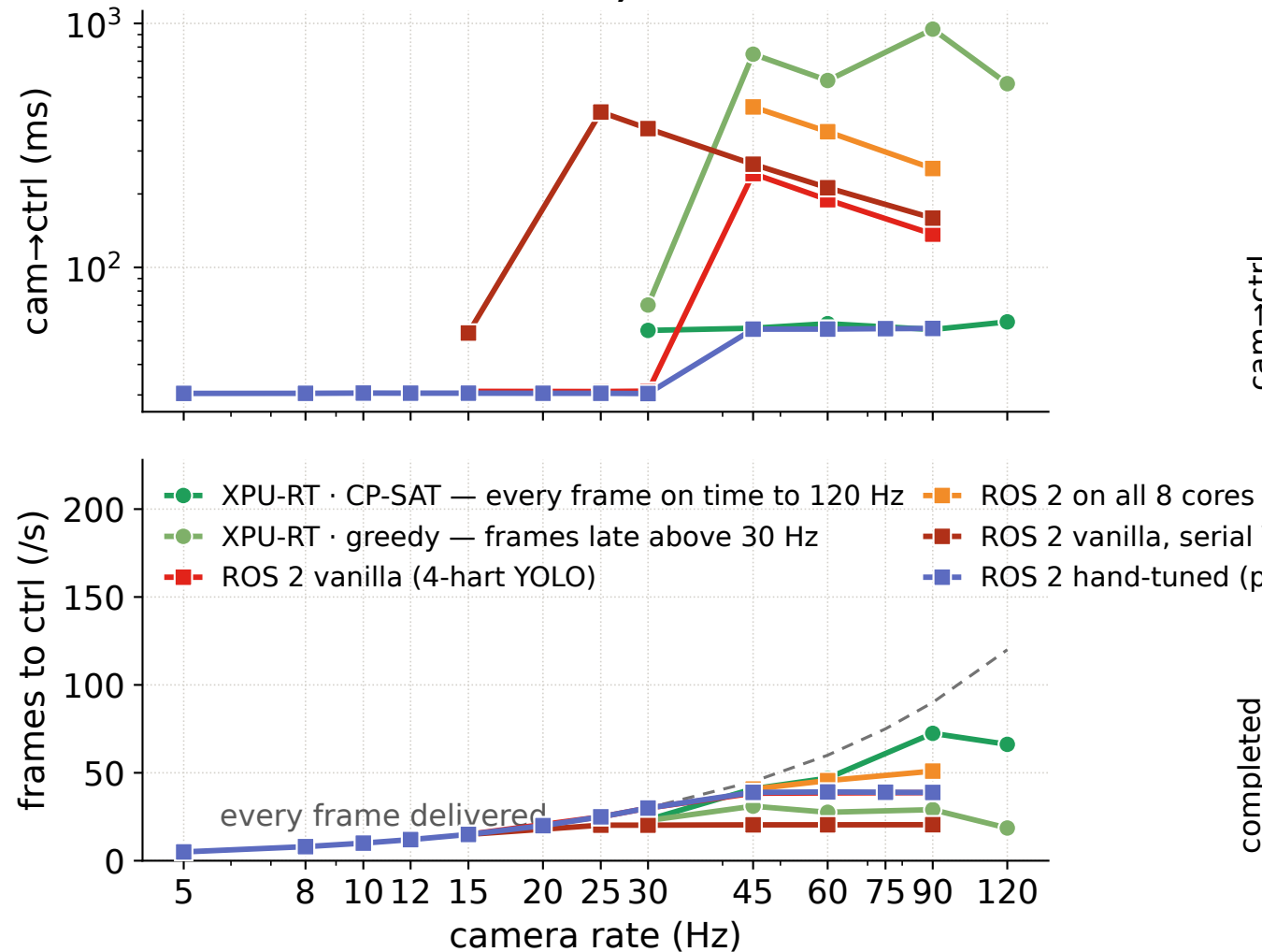
(a) Camera rate on the K1: camera→control latency and frames delivered, same kernels
