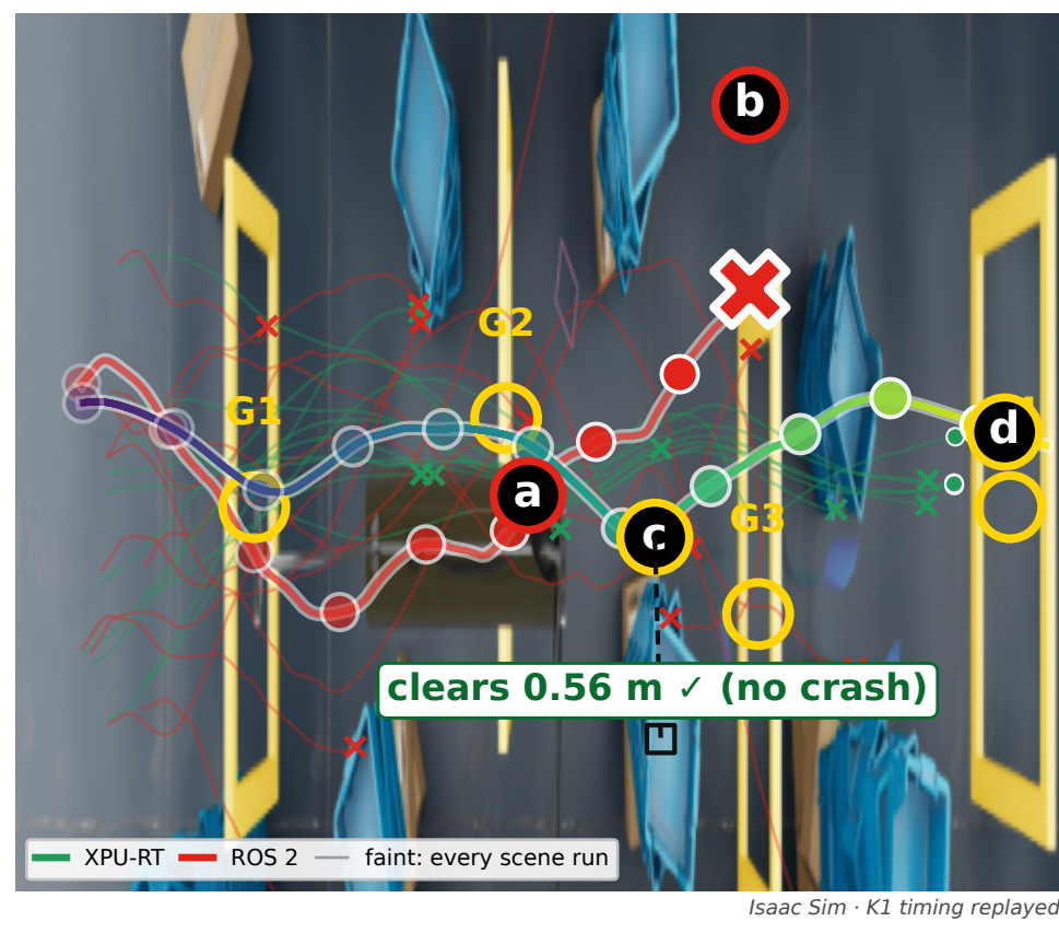
A · 36 Hz camera: XPU-RT solver-placed (100 Hz ctrl) vs ROS 2 on all 8 harts, chained (36 Hz); scene runs 4/12 vs 0/12
