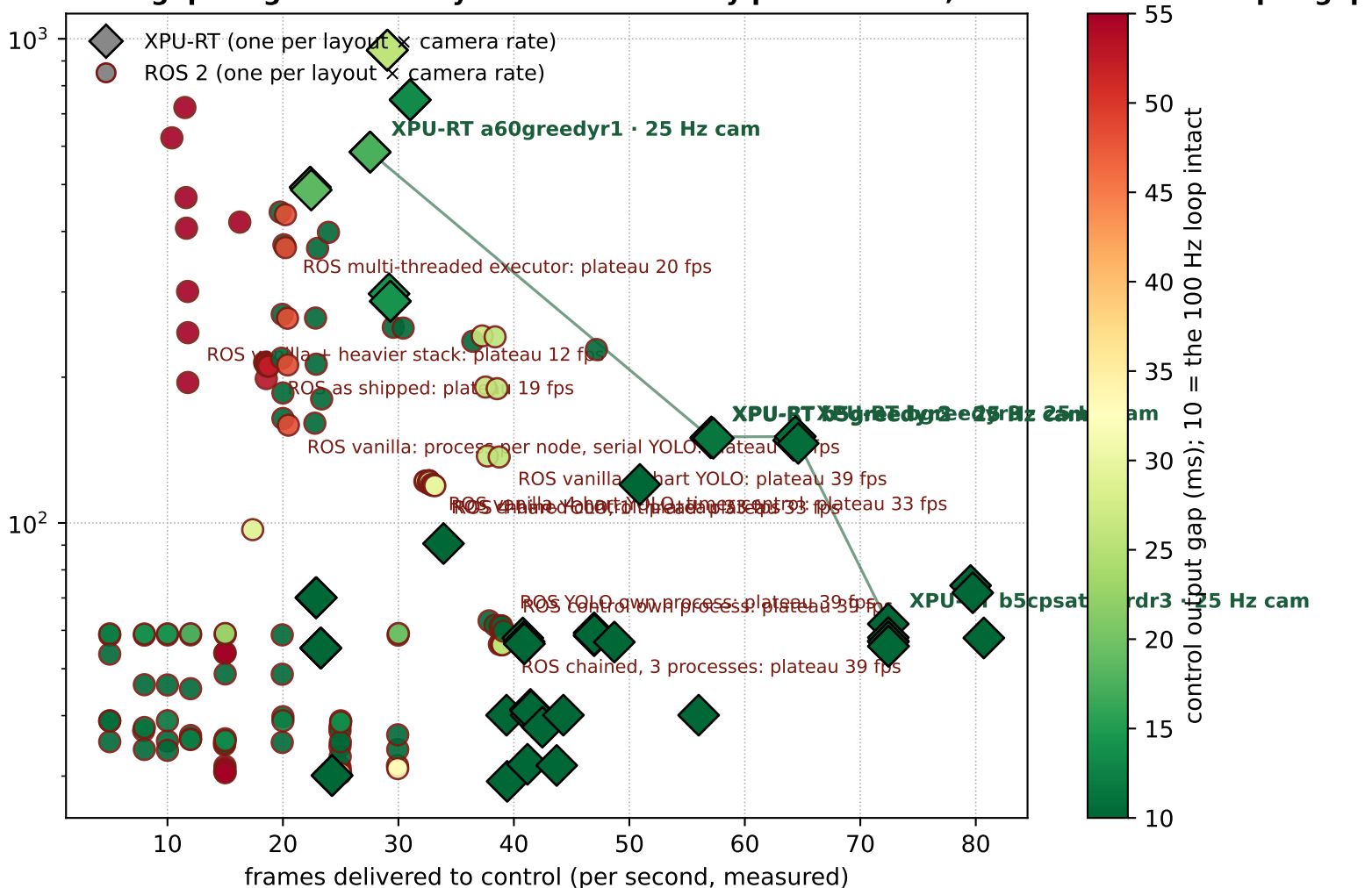
Throughput against latency on the K1 — every point is a run; colour = control-output gap
