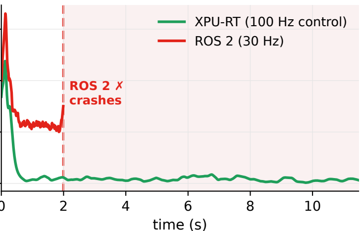
I Onboard K1 schedule, measured at the 30 Hz camera — XPU-RT · solver-placed CP-SAT schedule, conv on the IME places the kernels over all 8 harts: camera→control 27 ms, control every 10.0 ms, every frame on time · YOLO on 8 harts, 5 traced, nav on 5 harts, 2 traced, control on 1 hart ROS 2 · all 8 cores (5 processes · single executor · chained control · unpinned): camera→control 32 ms, control every 33.3 ms, 0/293 frames late · YOLO on 7 harts, 2 traced, nav on 1 hart, control on 1 hart
