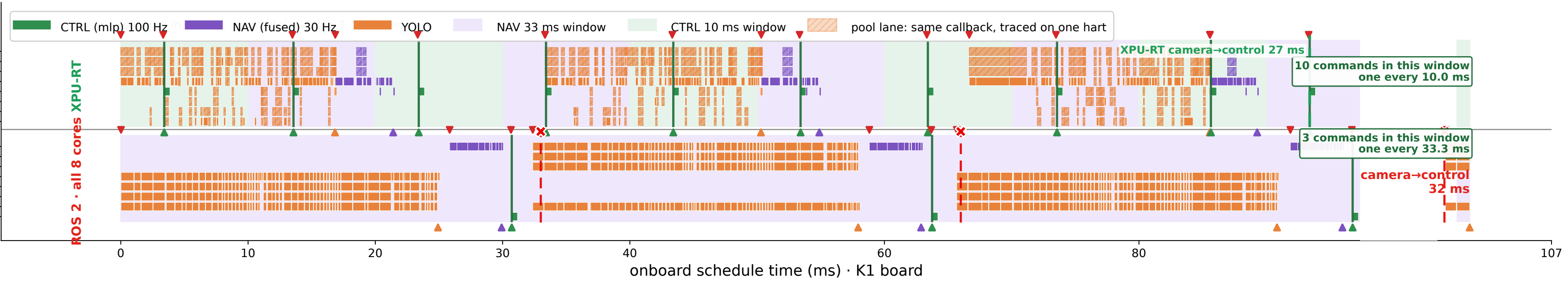
I Onboard K1 schedule, measured at the 30 Hz camera — XPU-RT · solver-placed CP-SAT schedule, conv on the IME places the kernels over all 8 harts: camera→control 27 ms, control every 10.0 ms, every frame on time · YOLO on 8 harts, 5 traced, nav on 5 harts, 2 traced, control on 1 hart ROS 2 · all 8 cores (5 processes · single executor · chained control · unpinned): camera→control 32 ms, control every 33.3 ms, 0/293 frames late · YOLO on 7 harts, 2 traced, nav on 1 hart, control on 1 hart
