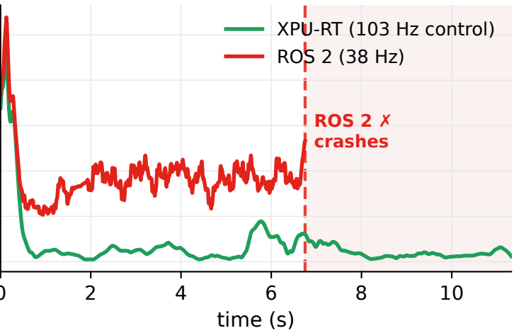
I Onboard K1 schedule, measured at the 45 Hz camera — XPU-RT · solver-placed CP-SAT schedule, conv on the IME places the kernels over all 8 harts: camera→control 27 ms, control every 9.9 ms, every frame on time · YOLO on 8 harts, control on 8 harts, nav on 8 harts ROS 2 · pinned (3 processes · single executor · chained control · pinned): camera→control 57 ms, control every 25.9 ms, 765/769 frames late · YOLO on 4 harts, 1 traced, control on 1 hart, nav on 1 hart
