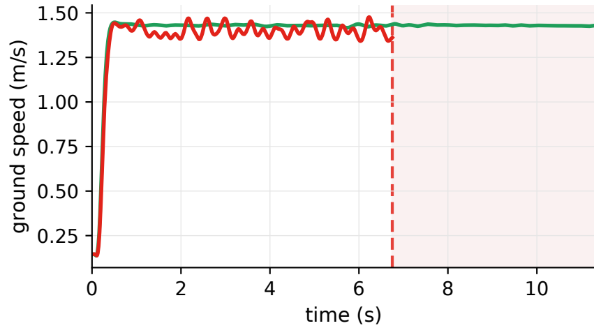
I Onboard K1 schedule, measured at the 45 Hz camera — XPU-RT · solver-placed CP-SAT schedule, conv on the IME places the kernels over all 8 harts: camera→control 27 ms, control every 9.9 ms, every frame on time · YOLO on 8 harts, control on 8 harts, nav on 8 harts ROS 2 · pinned (3 processes · single executor · chained control · pinned): camera→control 57 ms, control every 25.9 ms, 765/769 frames late · YOLO on 4 harts, 1 traced, control on 1 hart, nav on 1 hart
