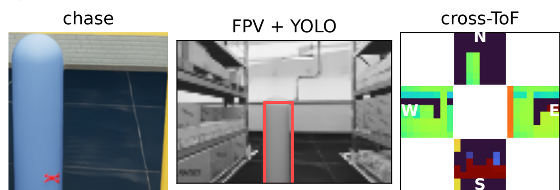
d XPU-RT 96 Hz · reaches gate · t=15.3s
