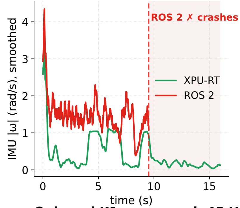
I Onboard K1, measured, 45 Hz camera — CP-SAT: 57 ms, every frame on time, control 10.0 ms · greedy: 748 ms, 44/44 late, control 13.2 ms ROS 2 8-core: 447 ms, control 16.6 ms · ROS 2 vanilla: 242 ms, control 25.6 ms
