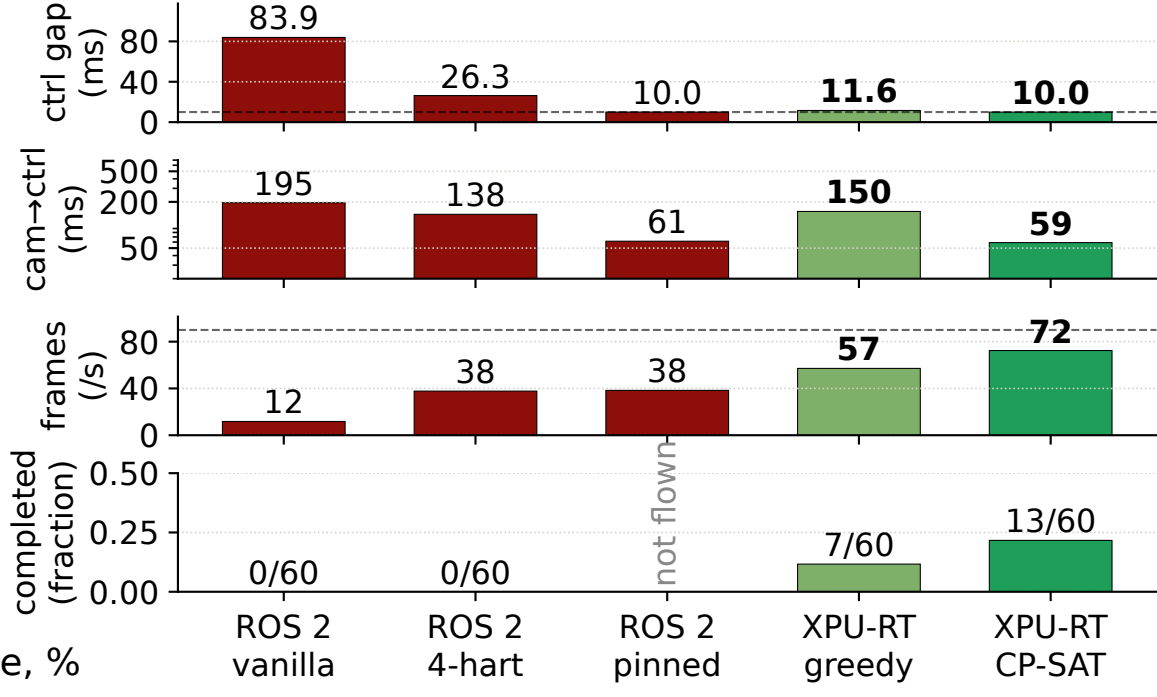
H Added load: 90 Hz camera + fnn_block + dronet on the same 8 harts
