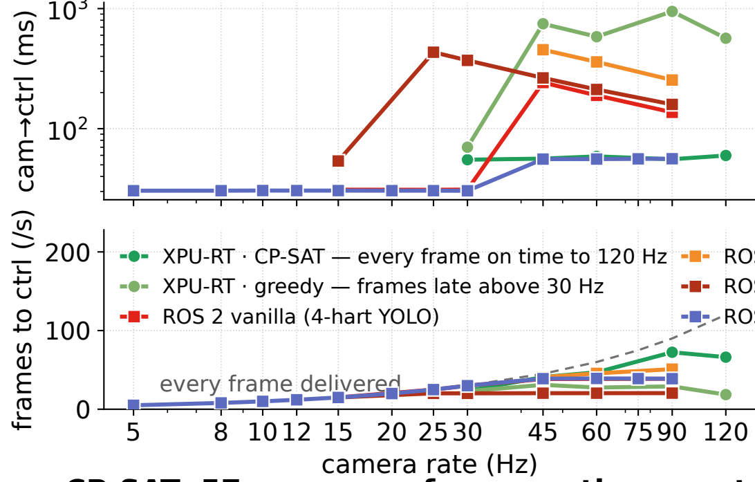
I Onboard K1, measured, 45 Hz camera — CP-SAT: 57 ms, every frame on time, control 10.0 ms · greedy: 748 ms, 44/44 late, control 13.2 ms ROS 2 8-core: 447 ms, control 16.6 ms · ROS 2 vanilla: 242 ms, control 25.6 ms
