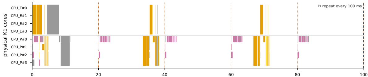
B After XPU-RT → ModelBlaster feedback — global optimum = 4.891 ms
