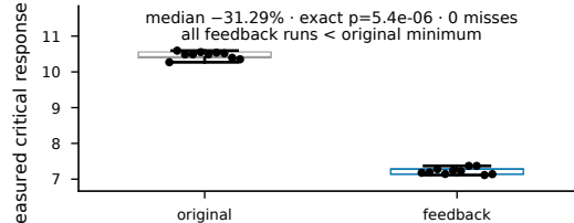
D 10 complete K1 runs per phase (SCHED_FIFO)
