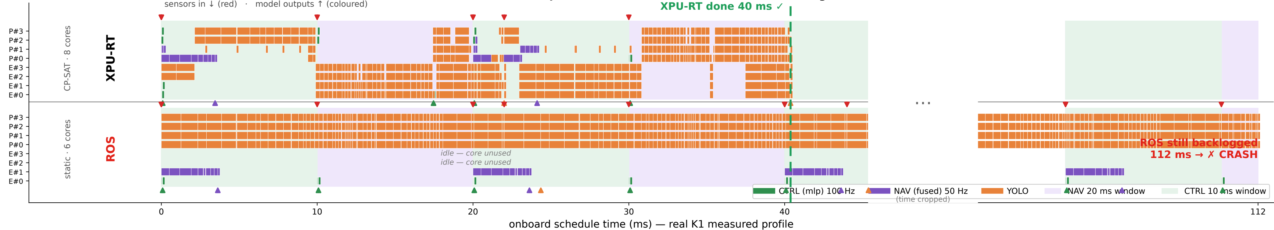
Combined onboard K1 schedule — XPU-RT balances 8 cores and fits the frame; ROS pins 6 cores, serial YOLO overruns → backlog → crash
