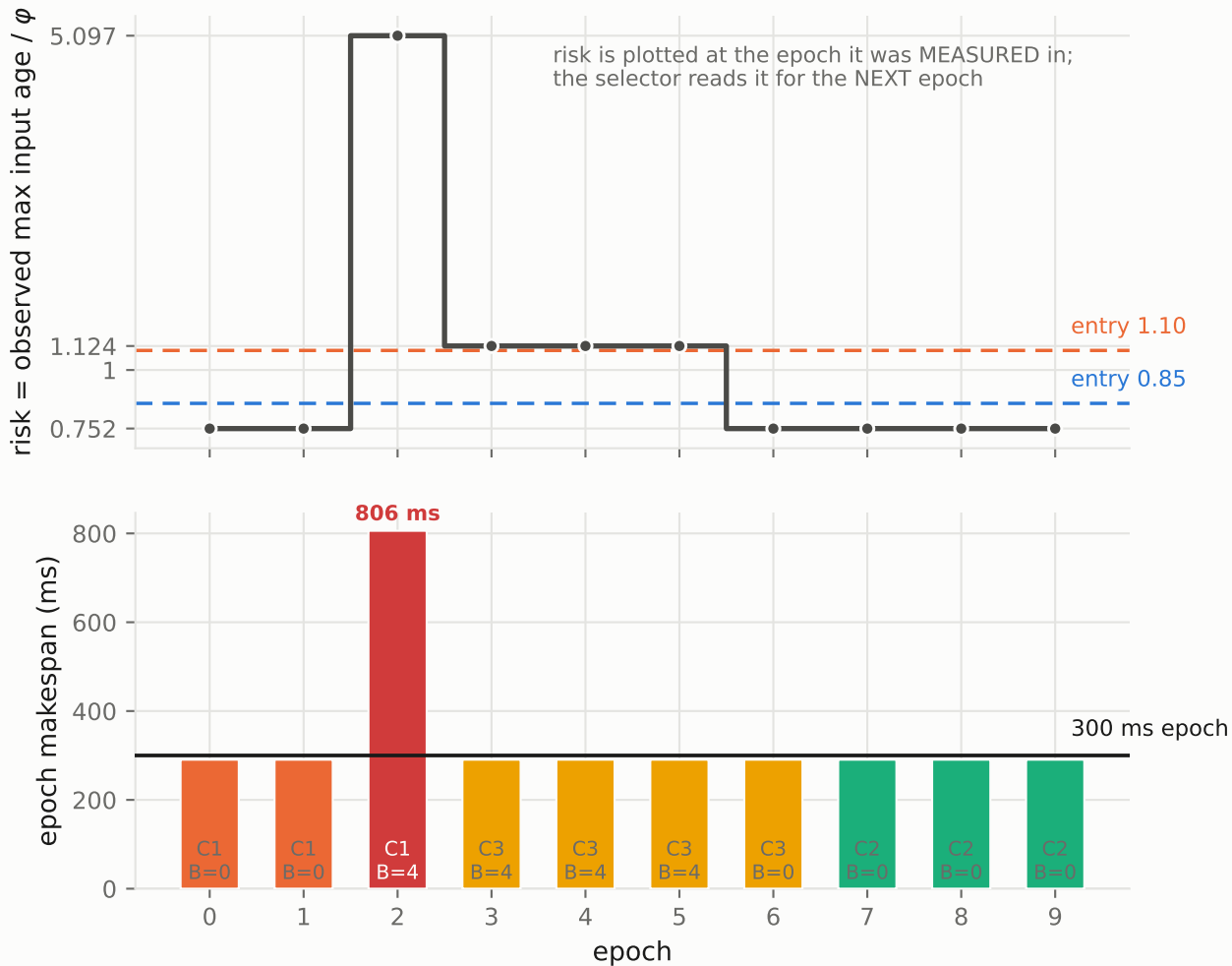
Plot 6 — the selector on `step`: reacting one epoch late costs one full epoch of a 2.7x overrun, then it escalates correctly
