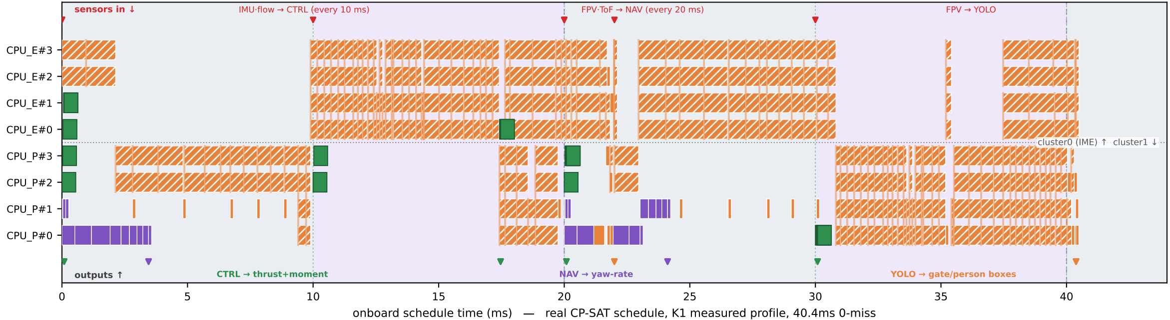
Onboard K1 warehouse schedule — CP-SAT balances CTRL 100Hz + NAV 50Hz + YOLO sharded across 8 cores (max hart 24ms vs greedy 38ms) · red = sensor in, coloured = output
