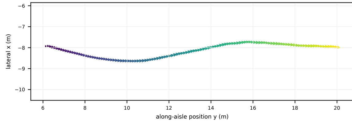
velocity — arrow direction = heading, length = forward speed (peak 1.31 m/s)
