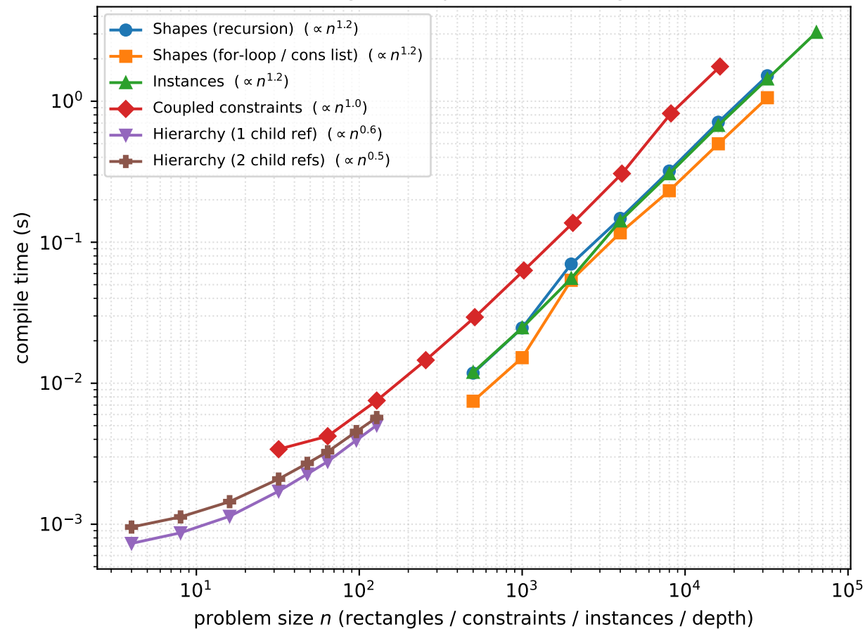
Argon compile-time scaling
