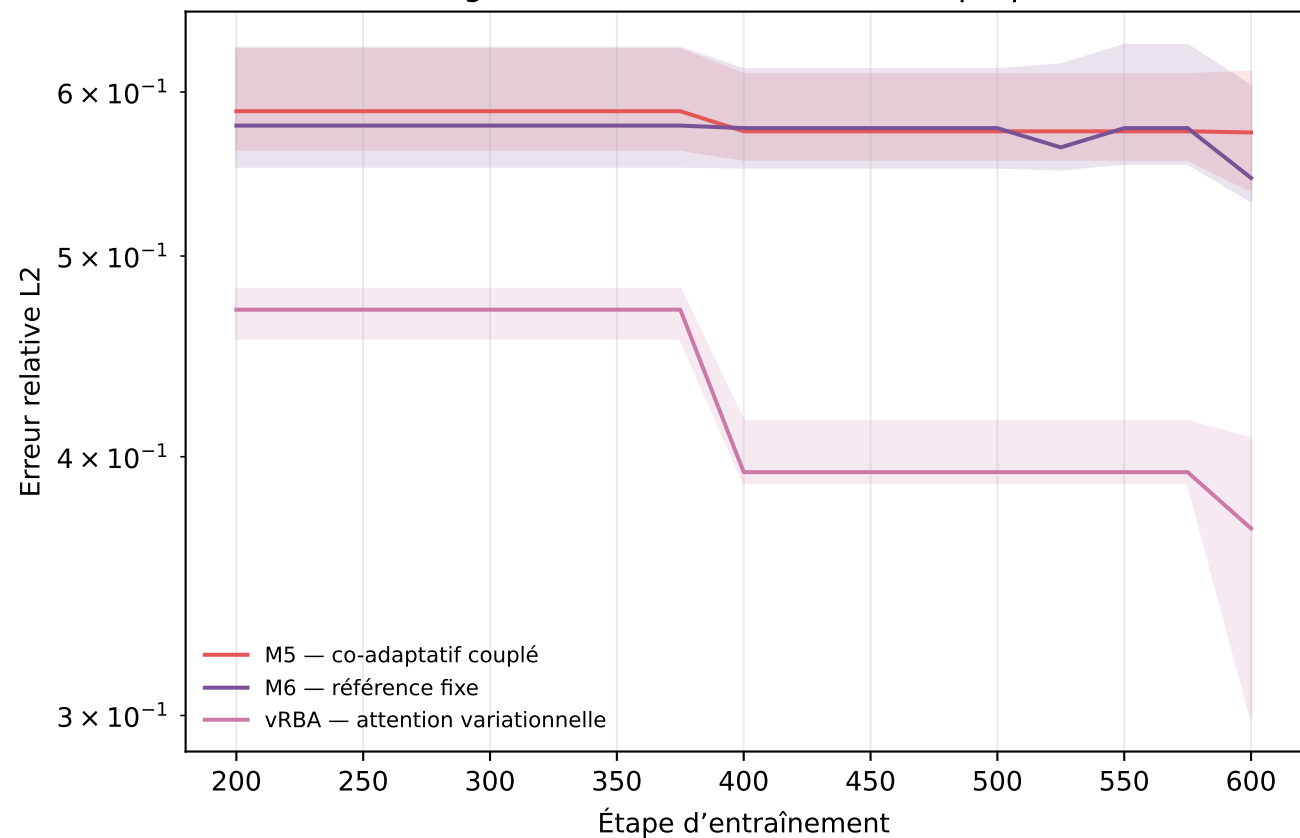
Burgers — vRBA, 13 observations propres
