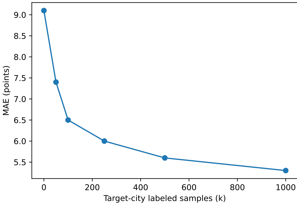
Transfer learning performance vs data size (pilot)
