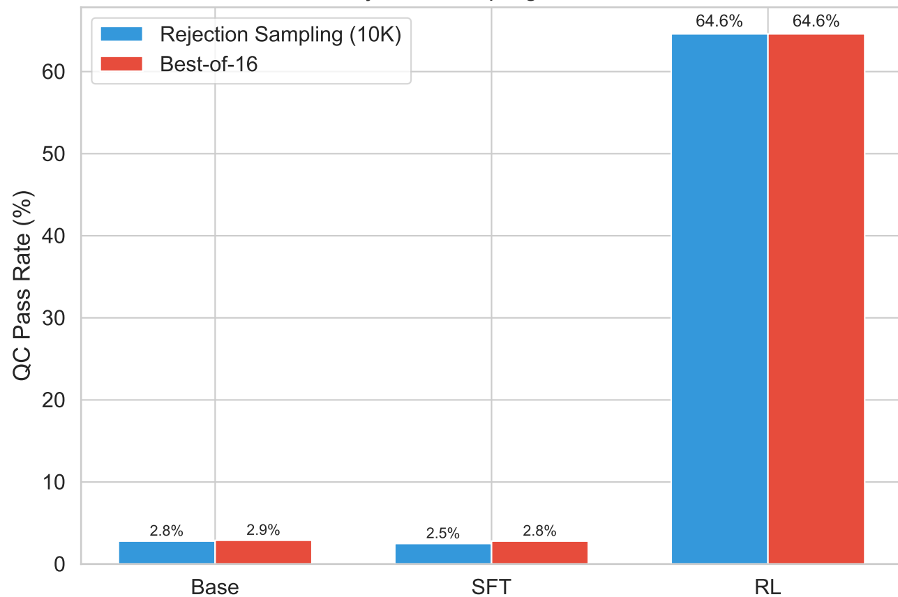
Rejection Sampling Baselines
