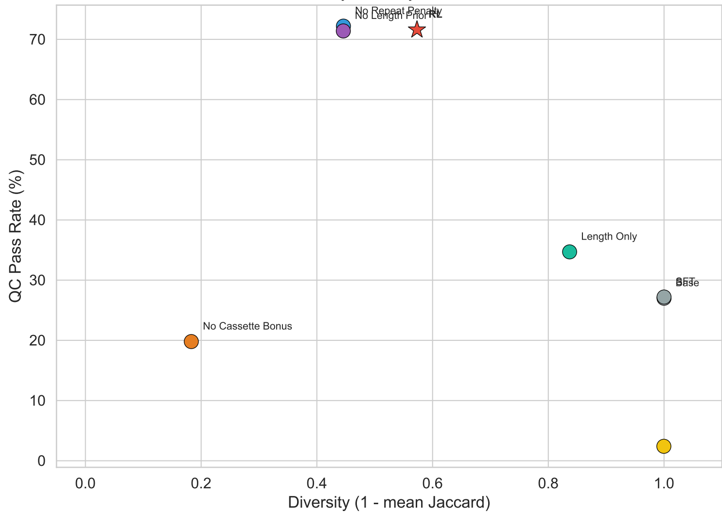
Quality-Diversity Tradeoff
