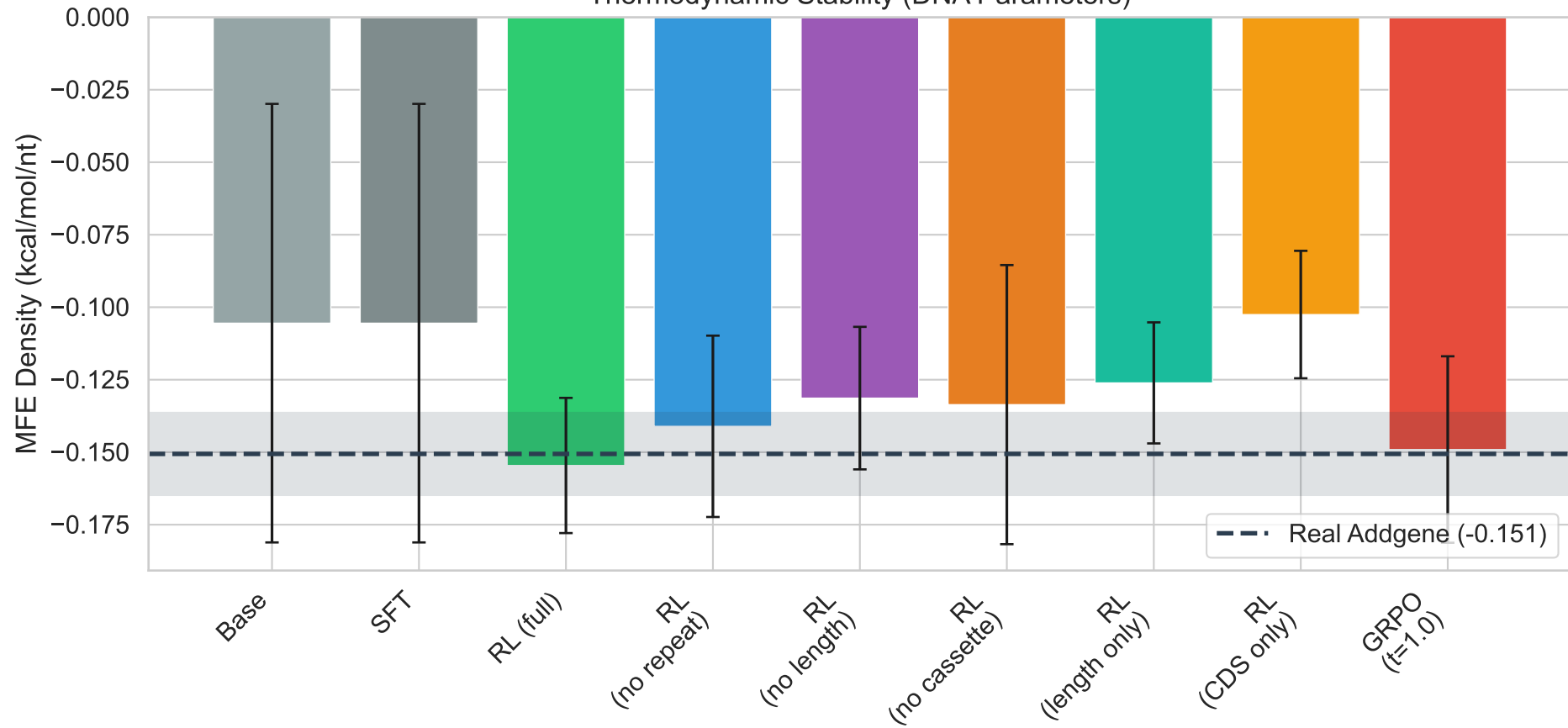
Thermodynamic Stability (DNA Parameters)
