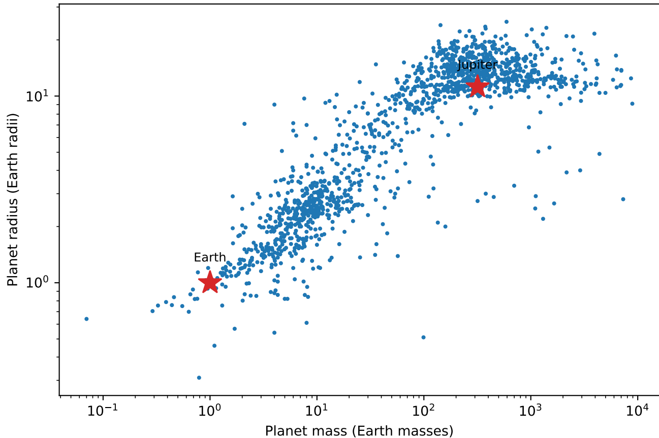
Exoplanet mass-radius diagram
