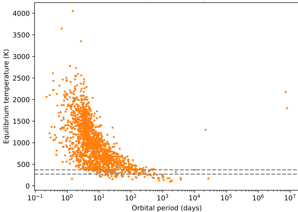
Period vs. equilibrium temperature
