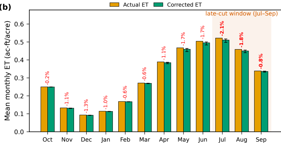
Mean monthly ET across the water year (all pooled)
