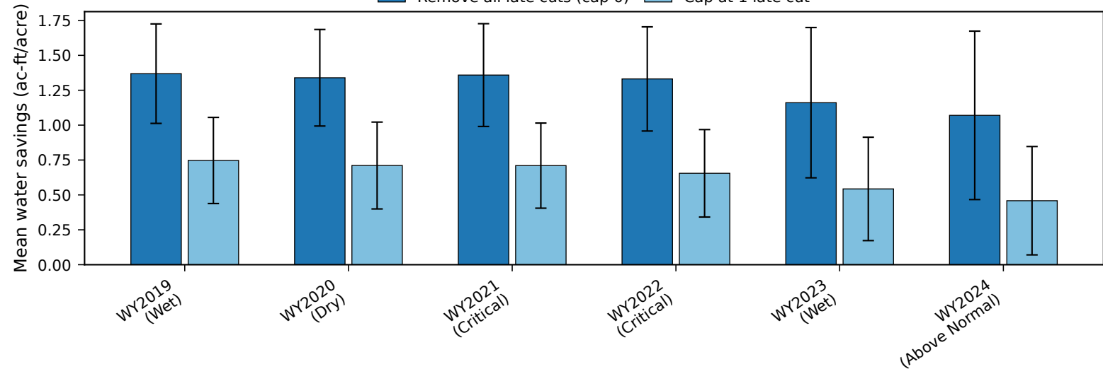
Water savings by water year — Actual ET, 10 counties pooled, mean per parcel-year
