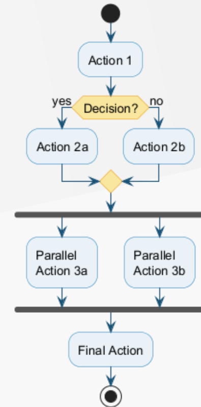
Activity Diagram Notation
