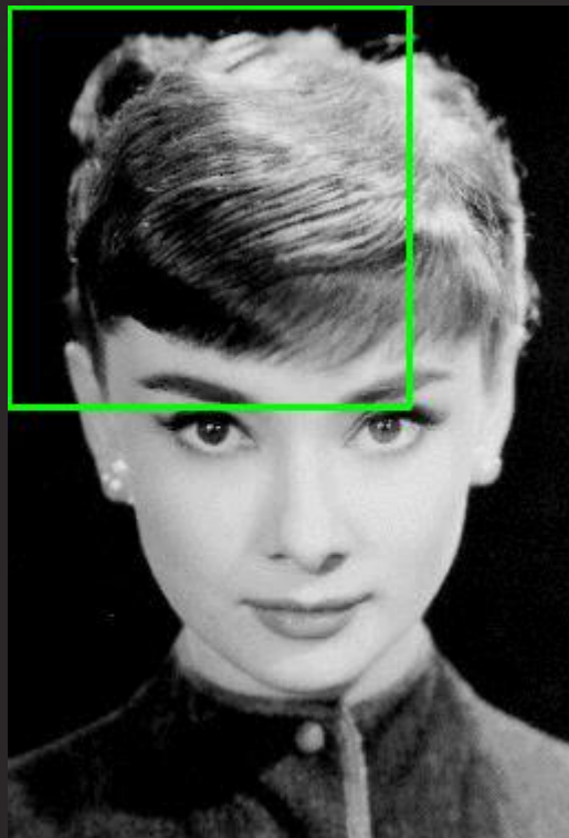
Sliding Window
