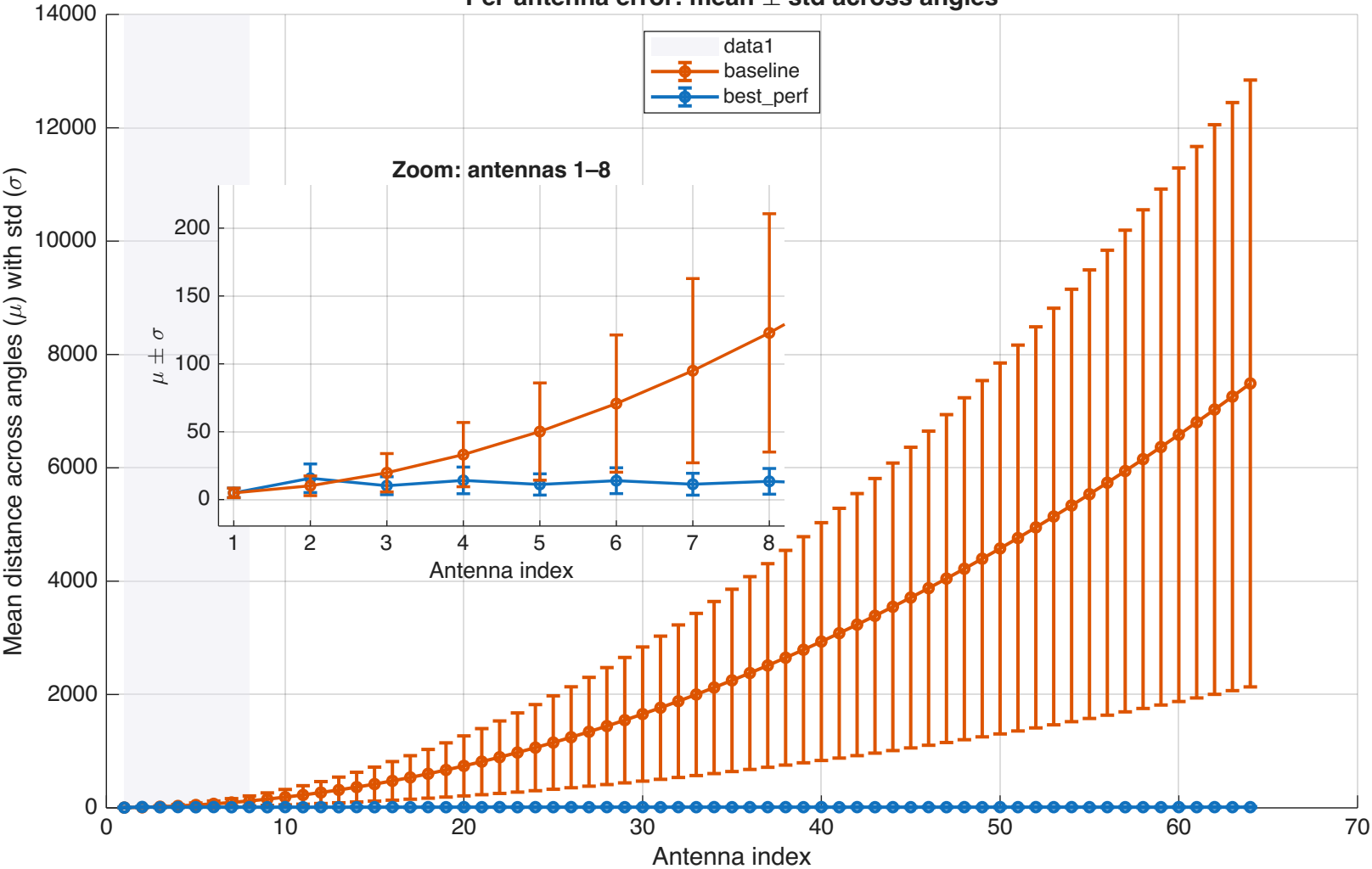
Per-antenna error: mean \pm std across angles
