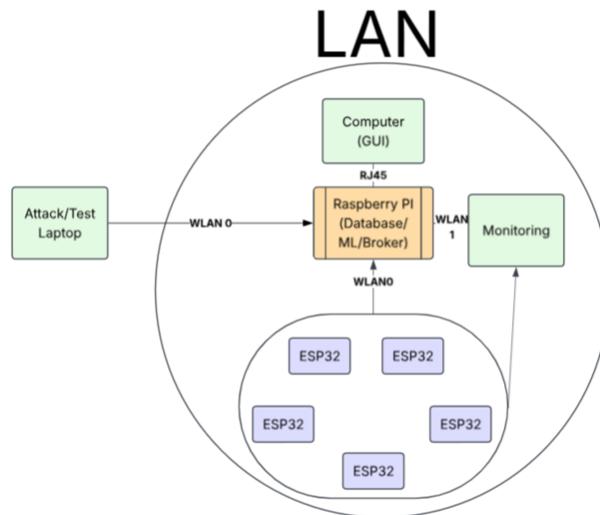
Figure 1: Top-down Network view
