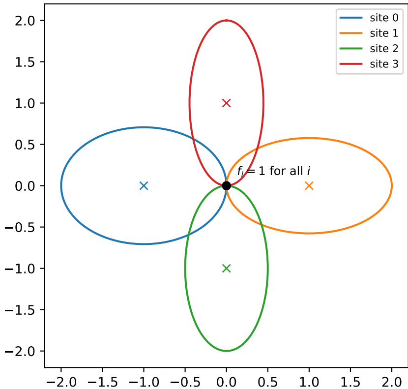
Degenerate configuration: all f_i = 1 at the origin
