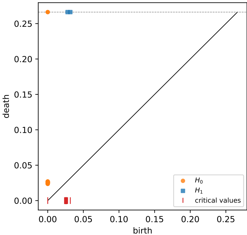
Persistence of the certified filtration
