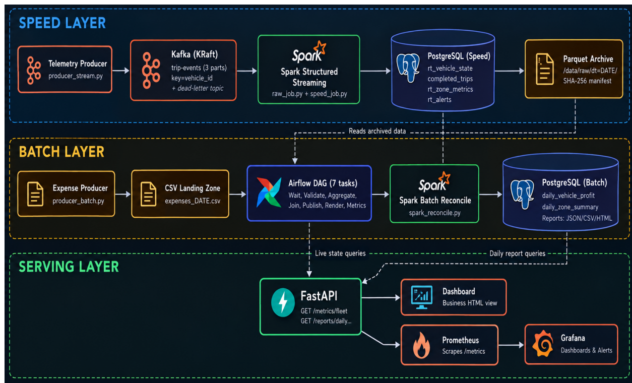
Figure 1. Delivered local Lambda architecture. Kafka feeds independent speed and raw consumers; PostgreSQL serves FastAPI and Prometheus is visualised in Grafana. The MinIO archive, database and checkpoints are operated as one dataset.
