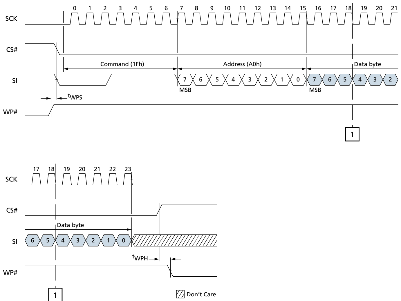
Figure 32: WP# Timing
