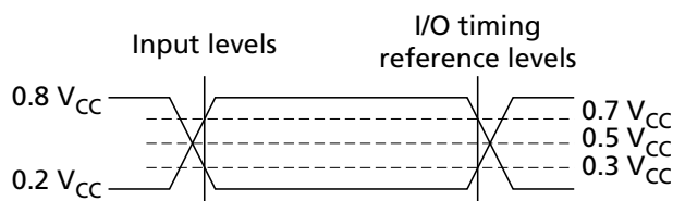
Figure 31: AC Measurement I/O Waveform
