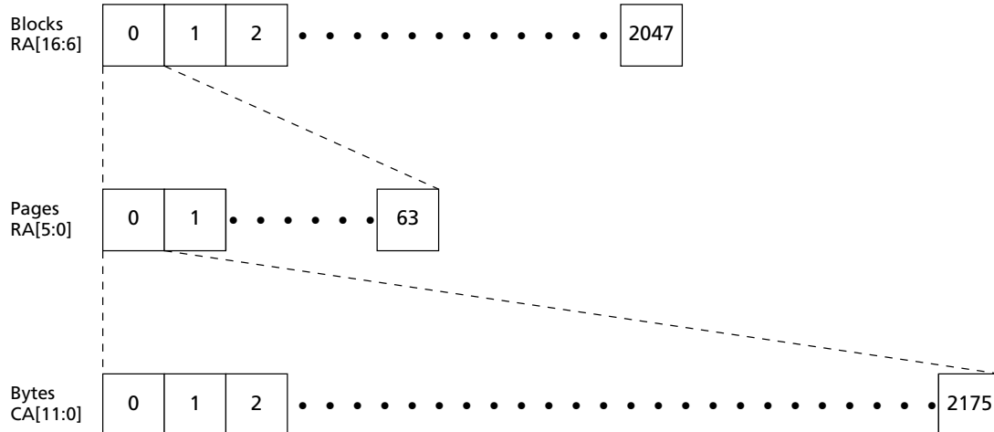
Figure 5: Memory Map
