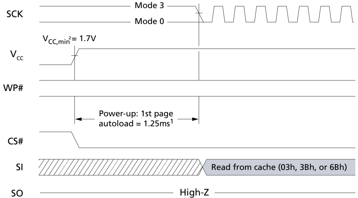
Figure 30: Automatic Device Initialization
