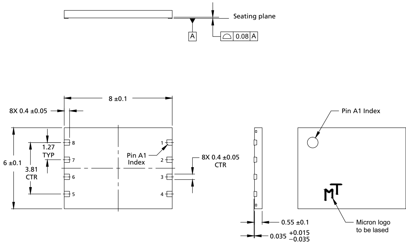
Figure 36: 8-pin U-PDFN (MLP8) 8mm x 6mm x 0.65mm – Package Code: WB
