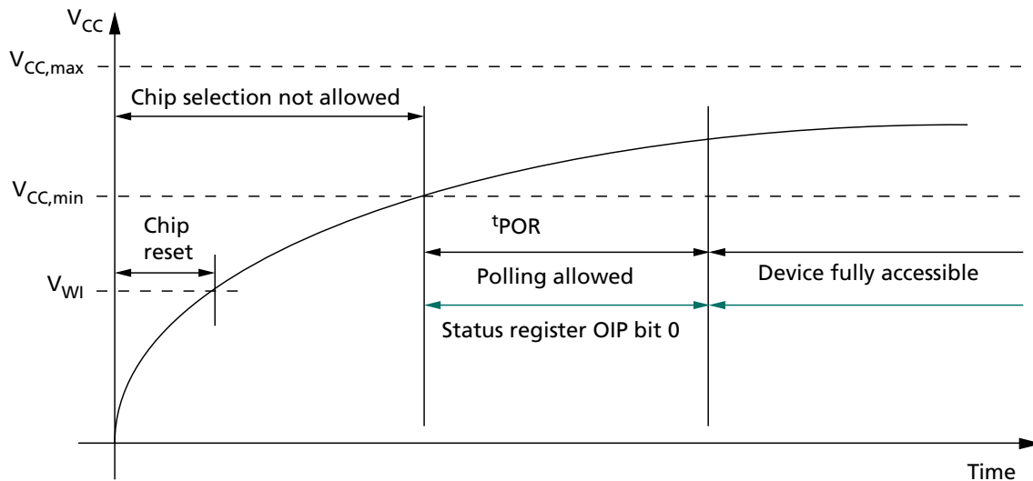
Figure 29: SPI Power-Up
