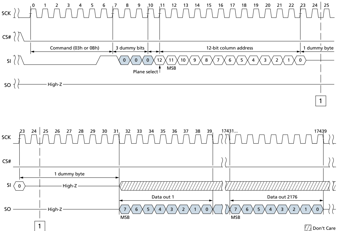
Figure 13: READ FROM CACHE (03h or 0Bh) Timing
