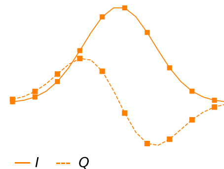
Gaussian DRAG-L
